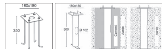
ARC.9120.xx Grondanker
