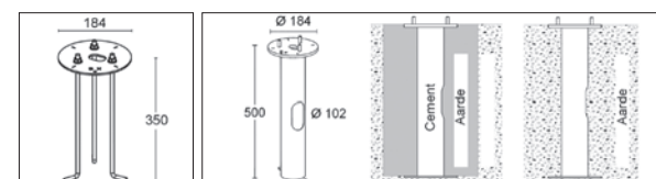
ARC.9100.xx Grondanker
