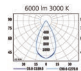
ELP.81 Medium breed stralend
