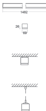
ELP.84 Corridor/gangpad
